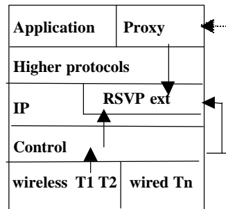
Figure 2: Mobile Node
